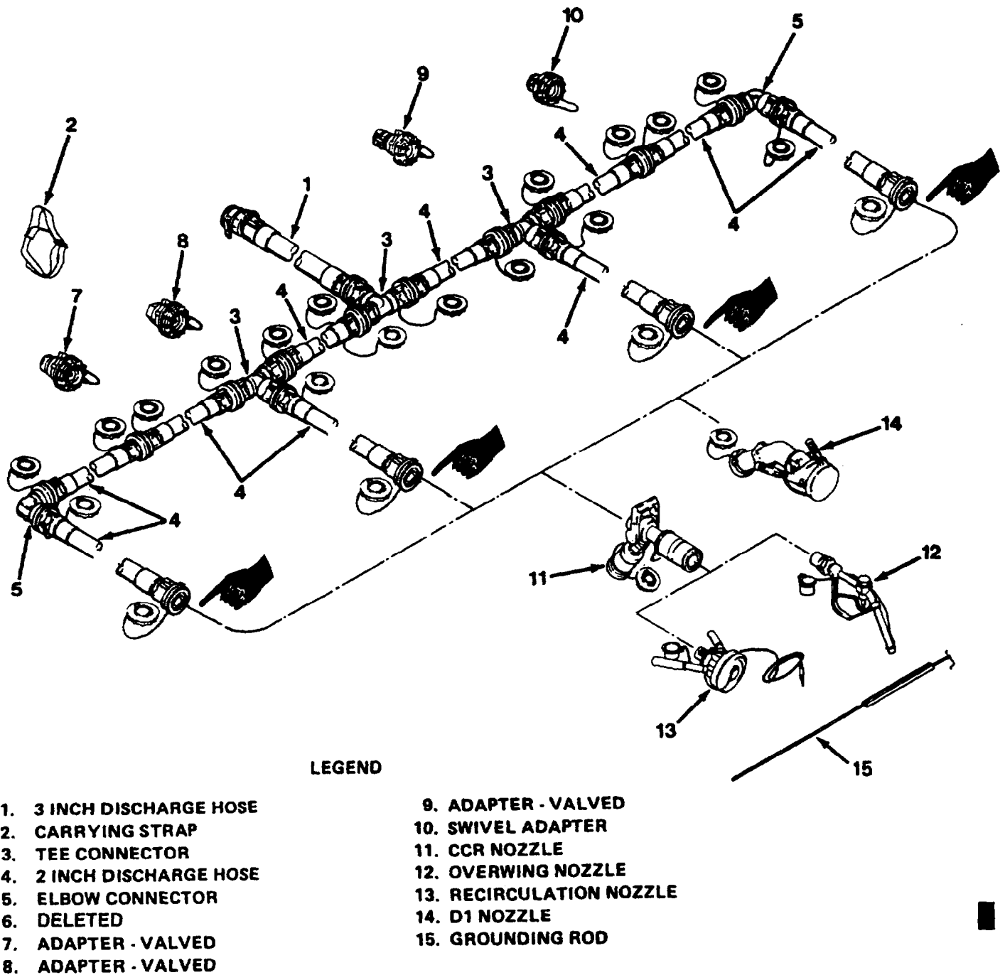
Figure 1-1. HEMTT Tanker Aviation Refueling System (HTARS)
