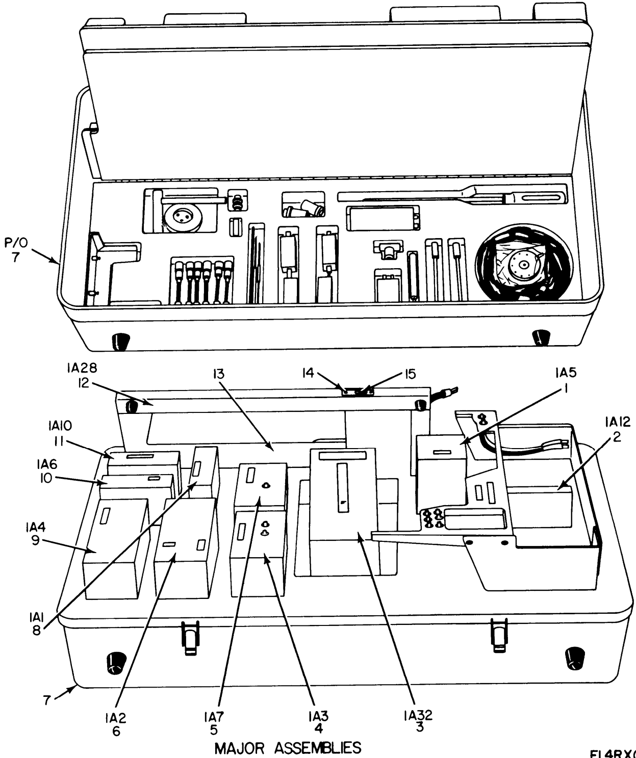
Figure 1. Maintenance Kit, Electronic Equipment MK-722/URC (1) (Sheet 1 of 2).
