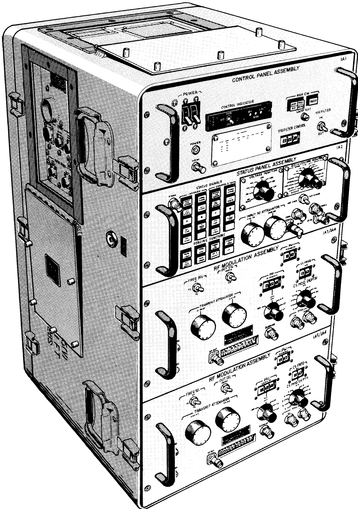
TEST SET, COUNTERMEASURES SET TS-3615/ALQ-136(V) (BENCH TEST SET)
